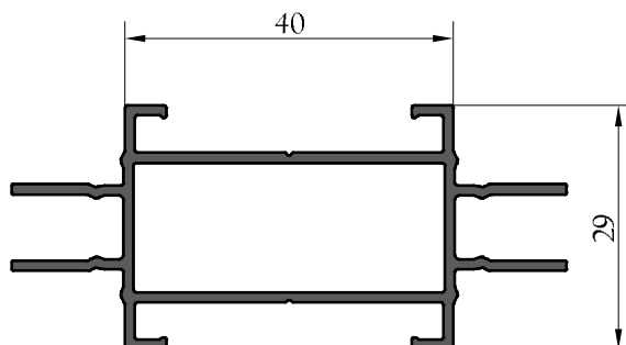
POTEAU
