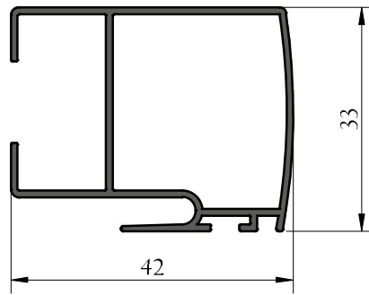
MONTANT CENTRAL SIMPLE
