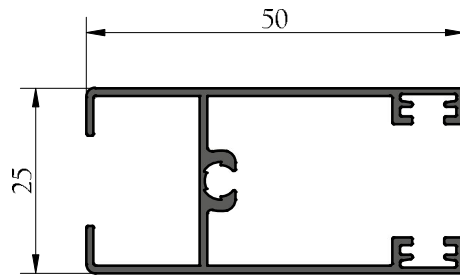
TRAVERSE
