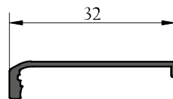
COUVRE JOINT
