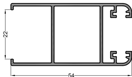
MONTANT LATERAL SIMPLE
