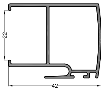
MONTANT CENTRAL SIMPLE
