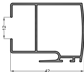
MONTANT CENTRAL
