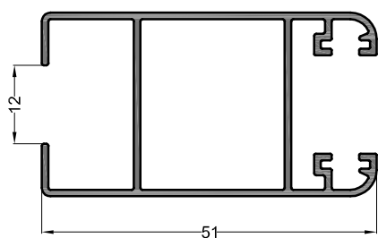
MONTANT LATERAL
