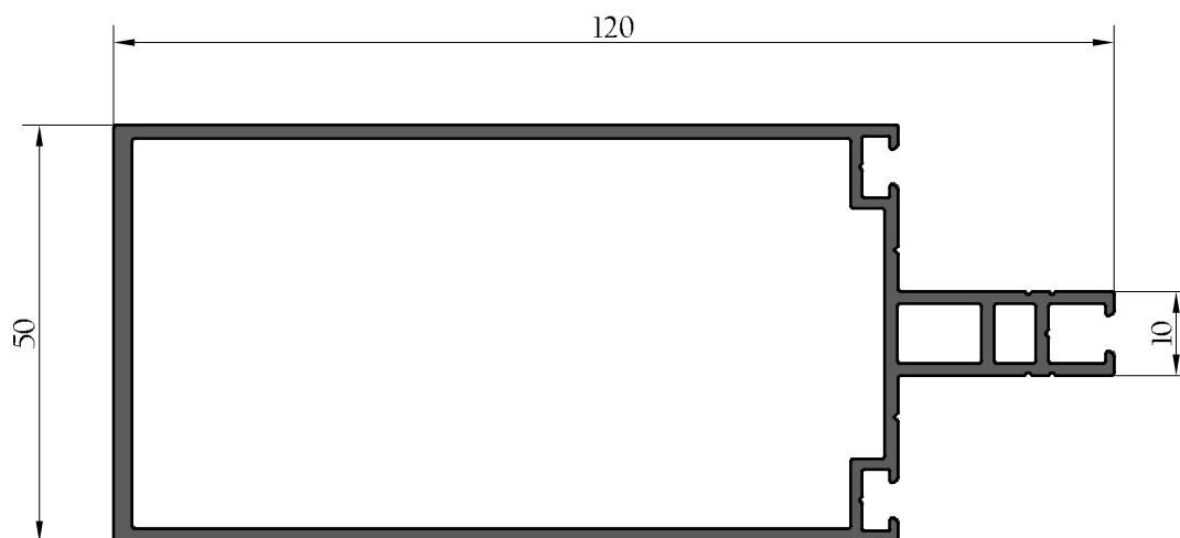
MENEAU-TRAVERSE 120 mm
