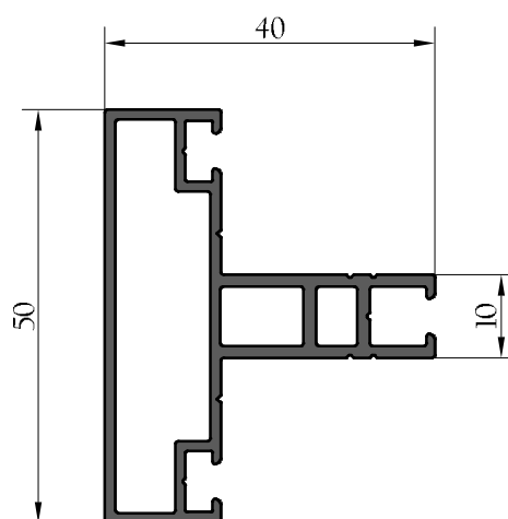
MENEAU-TRAVERSE 40 mm
