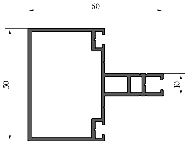
MENEAU-TRAVERSE 60 mm
