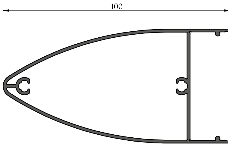
CAPOT OGIVE
