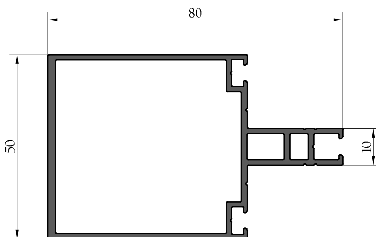
MENEAU-TRAVERSE 80 mm.
