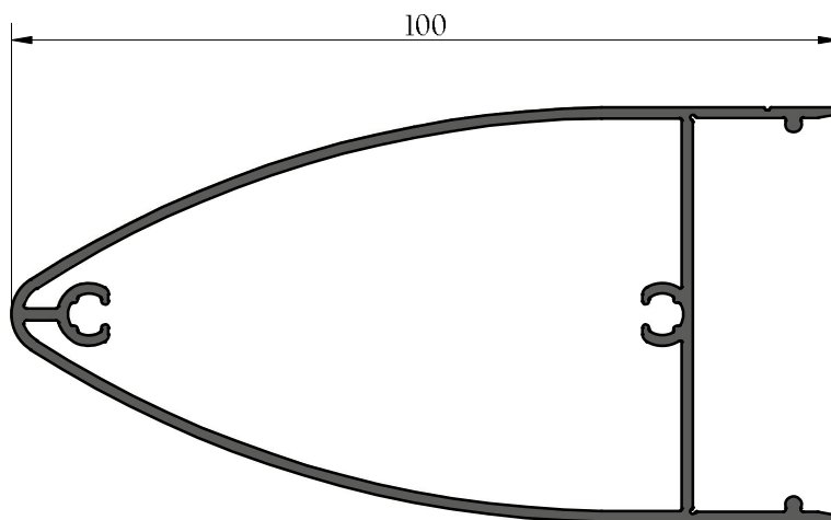
CAPOT OGIVE
