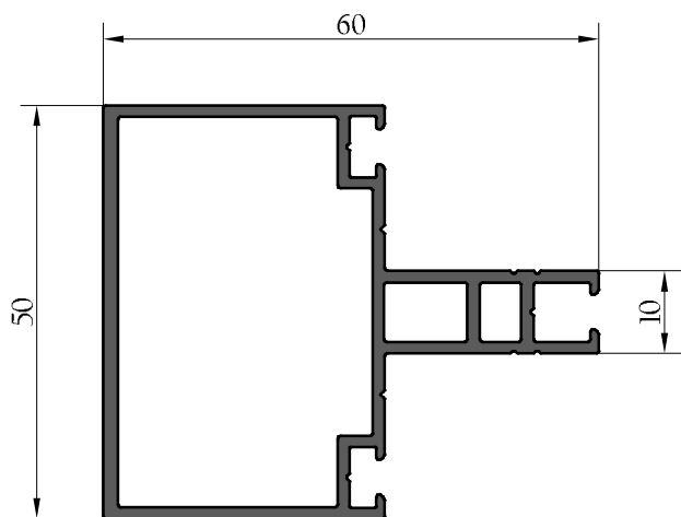
MENEAU-TRAVERSE 60 mm
